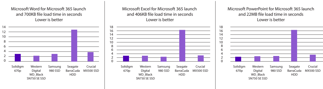
[Figure 11. Application launch and file-load times for Microsoft Word for Microsoft 365, Microsoft Excel for Microsoft 365, and Microsoft PowerPoint for Microsoft 365]
