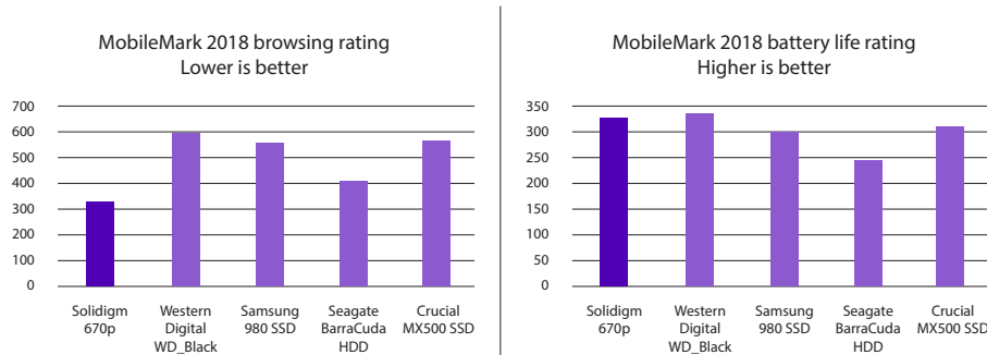
[Figure 9. MobileMark 2018 web browsing and battery life ratings]
