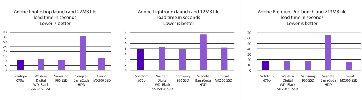
[Figure 10. Adobe Photoshop, Adobe Lightroom, and Adobe Premier Pro launch and file-load test results]
