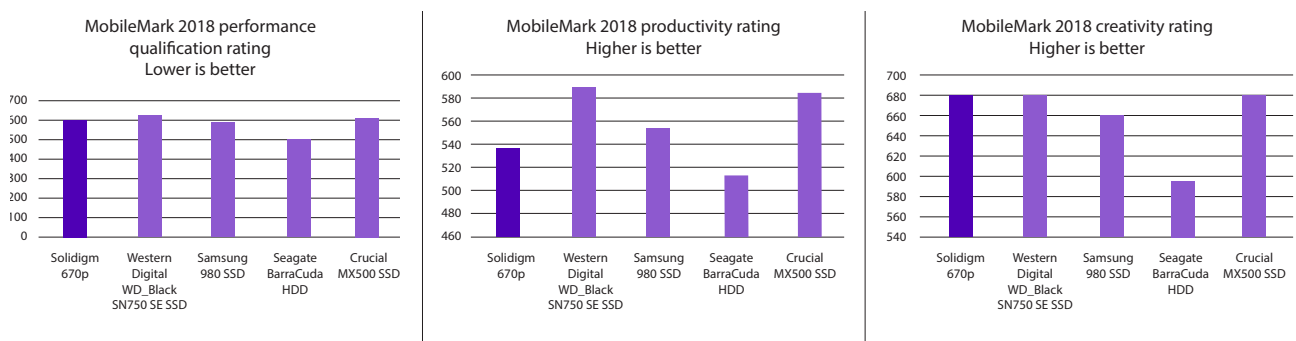
[Figure 8. MobileMark 2018 performance qualification, productivity, and creativity ratings]
